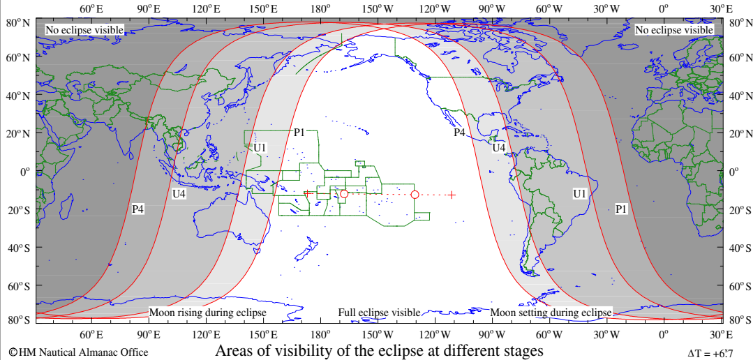
Areas of visibility of the eclipse at different stages
